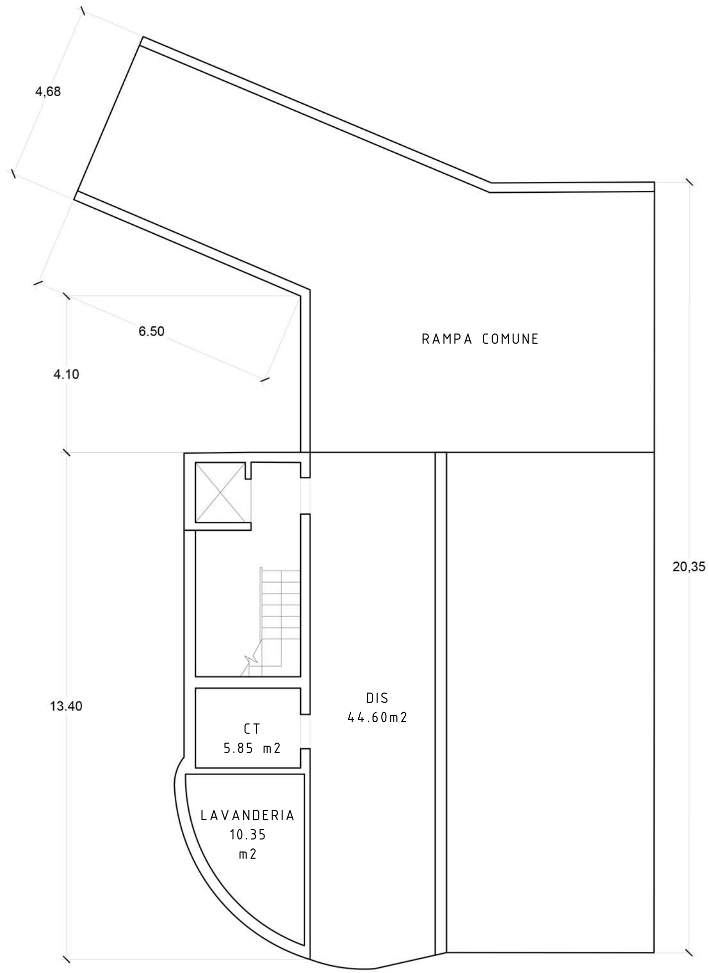
PIANO GARAGE sc. 1:100
